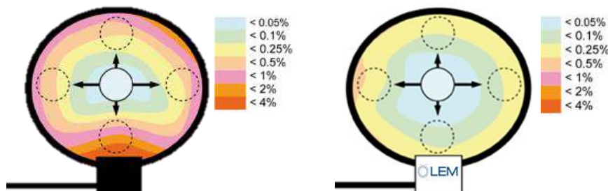
Figure 6: Rogowski coil accuracy comparison between a regular Rogowski coil and one using the LEM patented Rogowski coil clasp with primary conductor located at various positions inside the loop.
