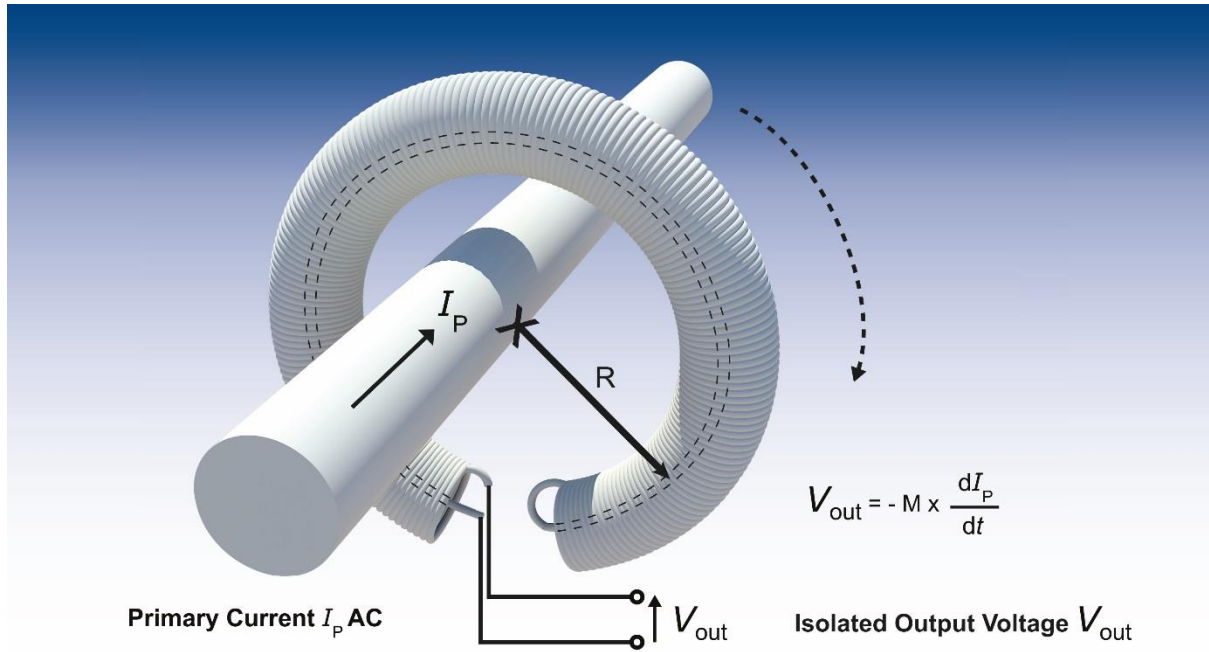
Figure 3: Rogowski Coil principle
