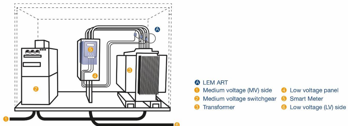
Figure 1: MV/LV Substation
