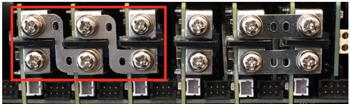
Figure 6-12. Modules connected in series with a series connection link
