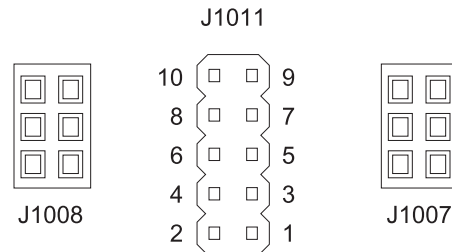
Figure 5-4. PMBus address header
