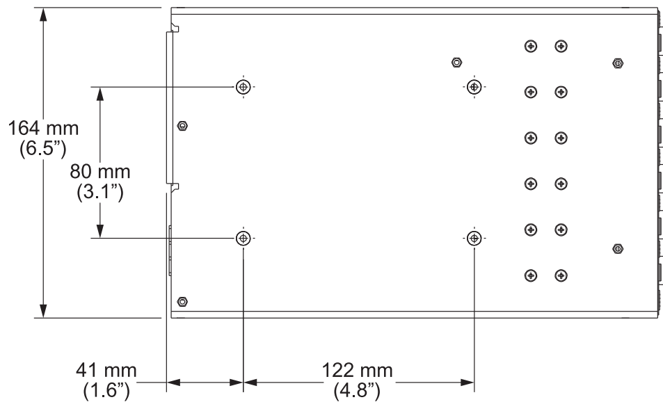
Figure 6-4. CoolX unit dimensions, bottom view
