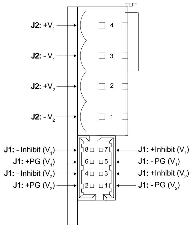
Figure 6-10. Dual module power terminals and signal connector
