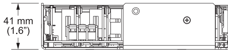
Figure 6-3. CoolX unit dimensions, AC input view
