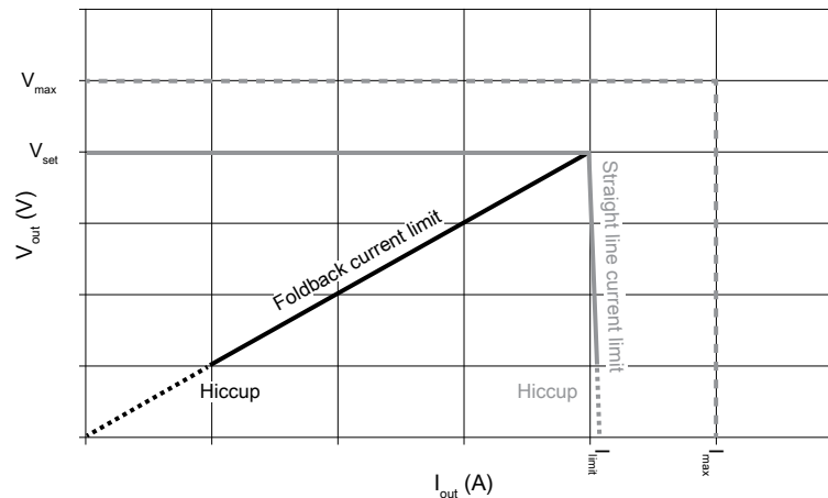
Figure 6-20. Current limit characteristics
