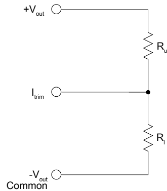
Figure 6-25. Foldback current limit circuit
