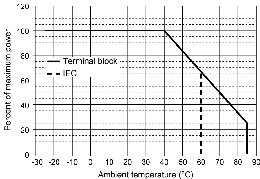
Figure 6-15. Chassis and module temperature derating
