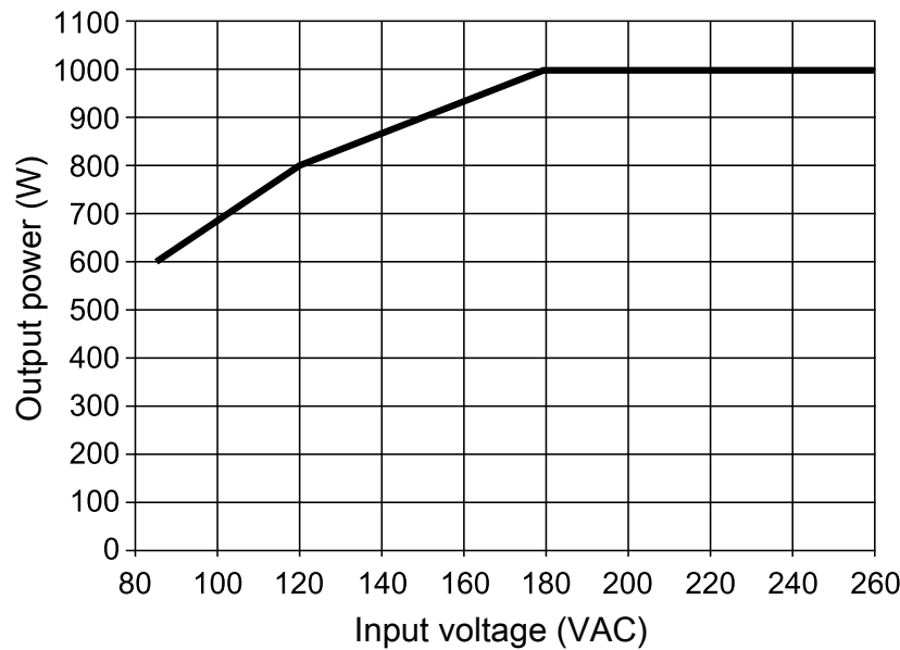
Figure 6-14. Chassis line derating with unit placed on steel baseplate
