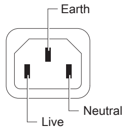
Figure 6-6. Optional IEC320 inlet terminal
