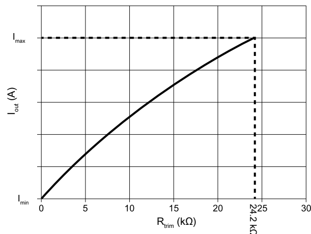
Figure 6-24. R_{trim} versus I_{out}
