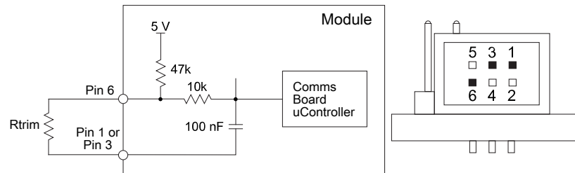
Figure 6-18. CoolMod wiring diagram for remote voltage setting using external resistance
