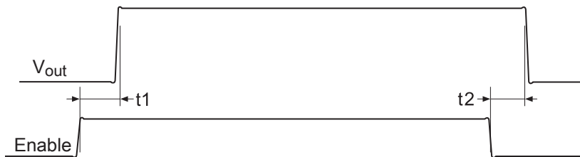
Figure 3-5. Module enable/disable timing
