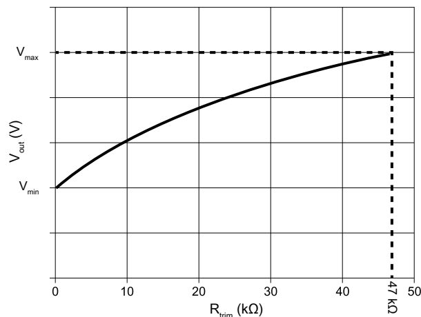
Figure 6-19. R_{trim} versus V_{out}
