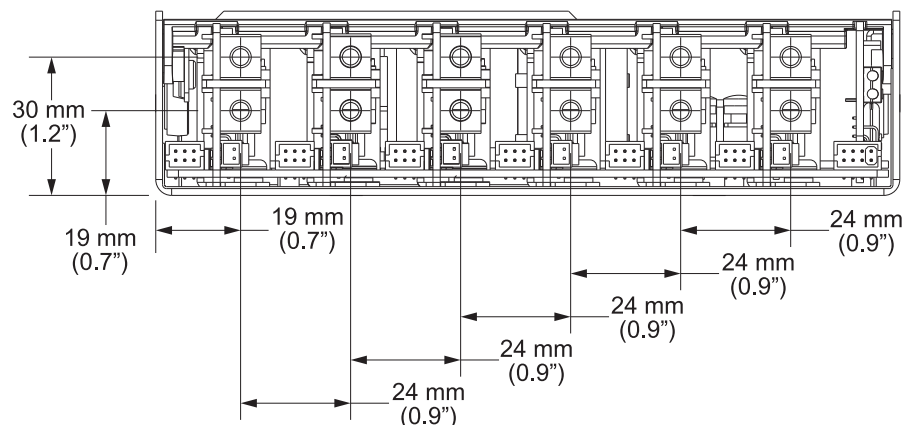
Figure 6-1. CoolX unit dimensions, DC outputs view
