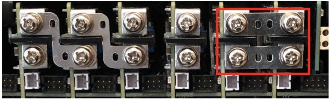
Figure 6-13. Modules connected in parallel with parallel connection links
