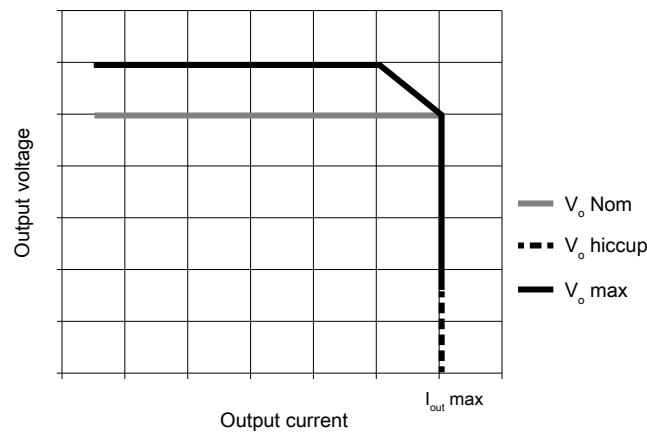
Figure 6-26. Current and power overload characteristics
