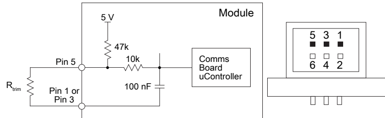
Figure 6-23. CoolMod wiring diagram for remote current setting using external resistance
