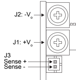
Figure 6-8. Standard and wide-trim module power terminals and sense connector
