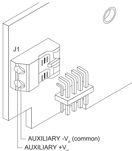
Figure 6-7. J1 auxiliary output connector
