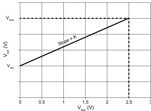
Figure 6-17. V_{trim} versus V_{out}
