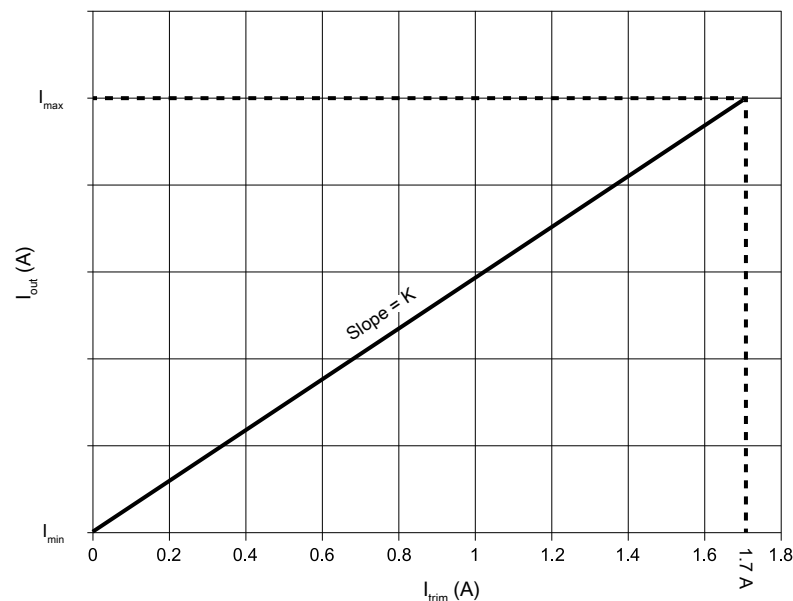
Figure 6-22. I_{trim} versus I_{out}
