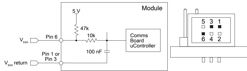
Figure 6-16. CoolMod wiring diagram for remote voltage setting using external voltage
