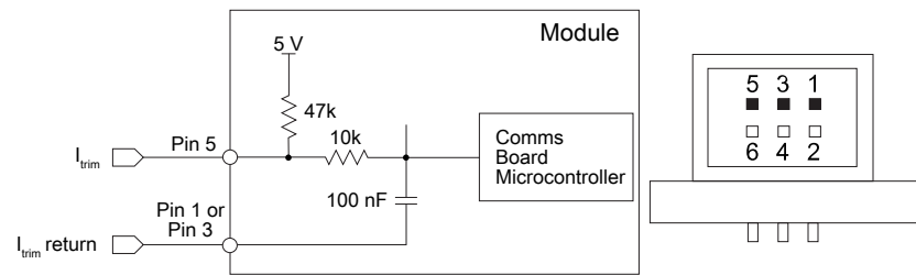
Figure 6-21. CoolMod wiring diagram for remote current setting using external voltage
