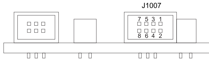
Figure 5-1. J1007 system signal connector
