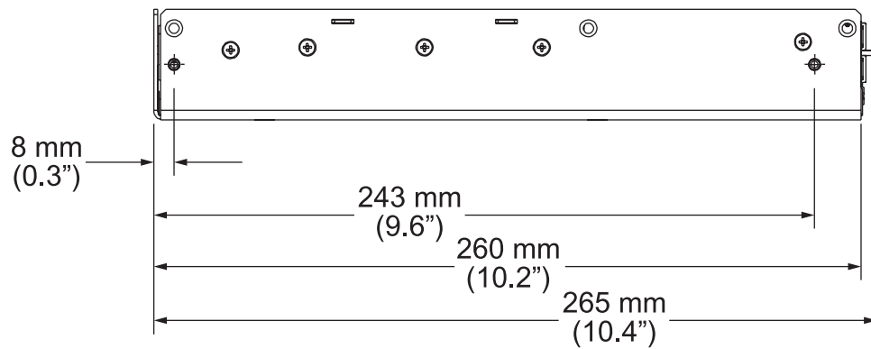
Figure 6-2. CoolX unit dimensions, side view
