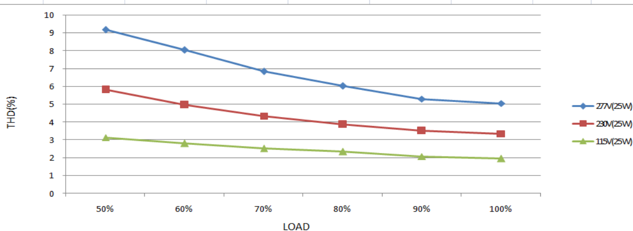
THD vs LOAD
