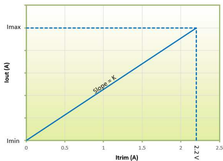
I_{trim} vs. I_{out}
