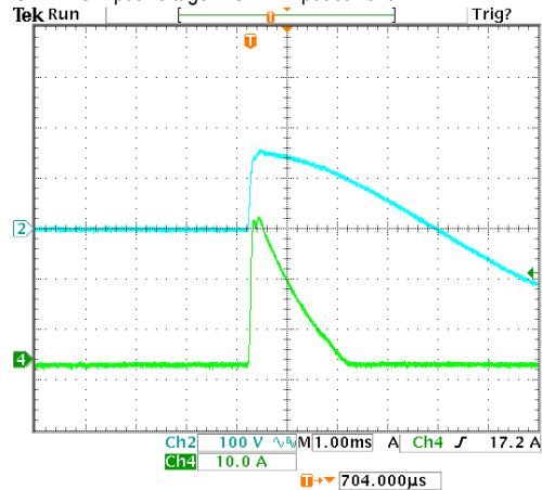
INPUT=115VAC/50HZ @ FULL LOAD
