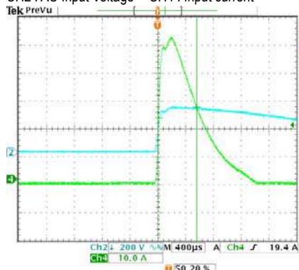
INPUT=230VAC/50HZ @ FULL LOAD
