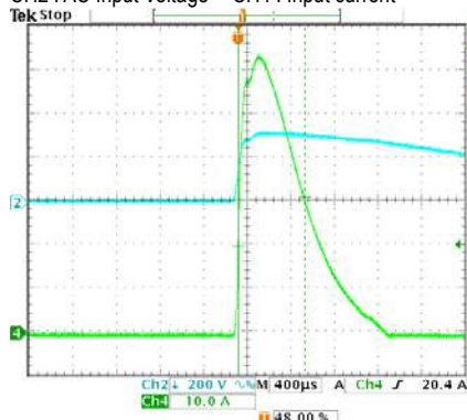
INPUT=230VAC/50HZ @ FULL LOAD
