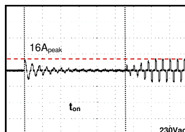
(Fig.8 inrush with ESB303)
