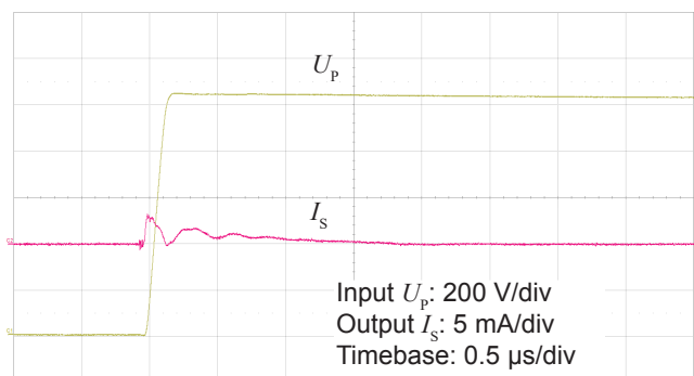
Figure 7: Detail of typical common mode perturbation (1000 V step with 6 kV/ \mu s, R_M = 100 \Omega )
