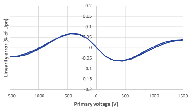
Figure 6: Typical linearity error at 25 °C
