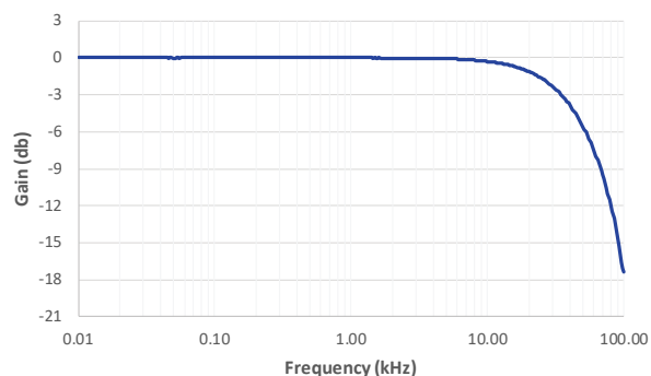
Figure 9: Gain function of frequency
