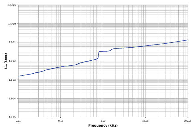
Figure 12: Typical total output RMS noise voltage U_{no} referred to primary with R_M = 50 \Omega
