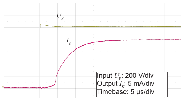
Figure 8: Typical step response (0 to 1000 V)
