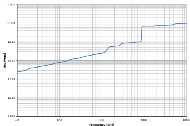
Figure 13: Typical total output RMS noise voltage U_{no} referred to primary with R_M = 50 \Omega
