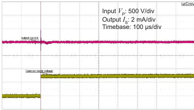
Figure 11: Typical common mode perturbation (750 V step with 6 kV/µs, R_M = 100 \Omega )
