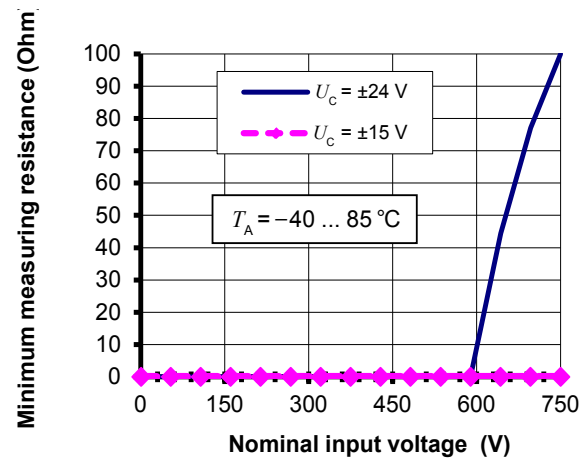
Figure 2: Minimum measuring resistance For T_A under 80 °C, the minimum measuring resistance is 0 \Omega whatever U_C
