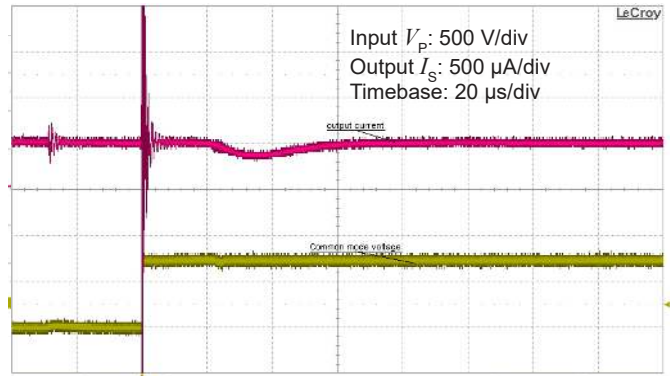
Figure 12: Detail of typical common mode perturbation (750 V step with 6 kV/µs, R_M = 100 \Omega )
