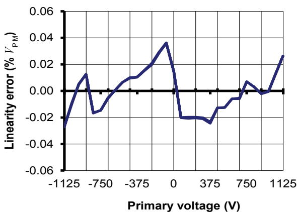
Figure 15: Typical linearity error at 25 °C
