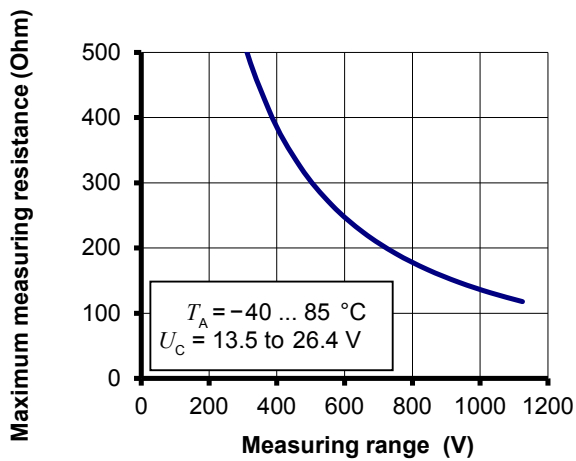
Figure 1: Maximum measuring resistance
