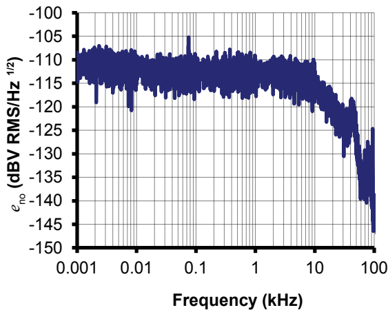
Figure 13: Typical output RMS noise voltage spectral density e_{no} with R_M = 50 \Omega
