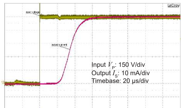
Figure 6: Typical step response (0 to 750 V)
