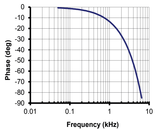
Figure 10: Typical frequency and phase response (detail)
