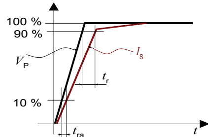
Figure 17: Response time t_r and reaction time t_{ra}
