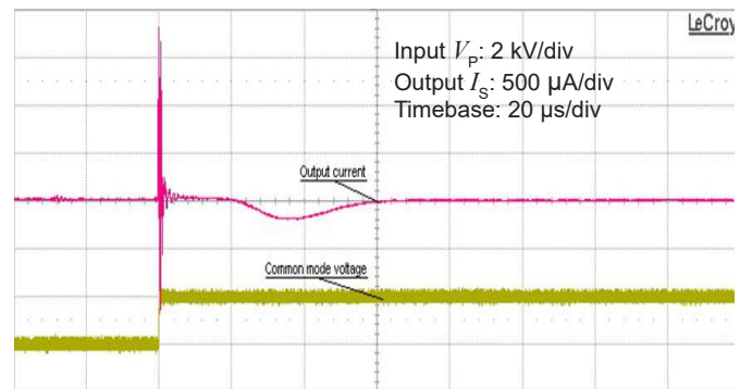
Figure 12: Detail of typical common mode perturbation (250 V step with 6 kV/μs, R_M = 100 \Omega )
