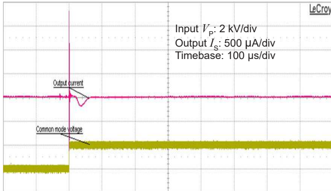
Figure 11: Typical common mode perturbation (250 V step with 6 kV/μs R_M = 100 \Omega )
