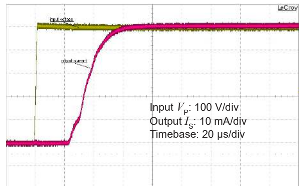
Figure 6: Typical step response (0 to 500 V)
