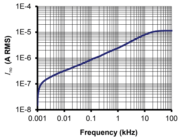
Figure 14: Typical total output RMS noise current with R_M = 50 \Omega ( f_c is upper cut-off frequency of bandpass, low cut off frequency is 1 Hz)
