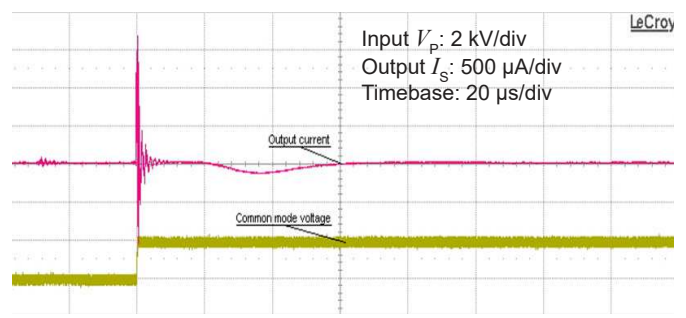
Figure 12: Detail of typical common mode perturbation (2000 V step with 6 kV/μs, R_M = 100 \Omega )
