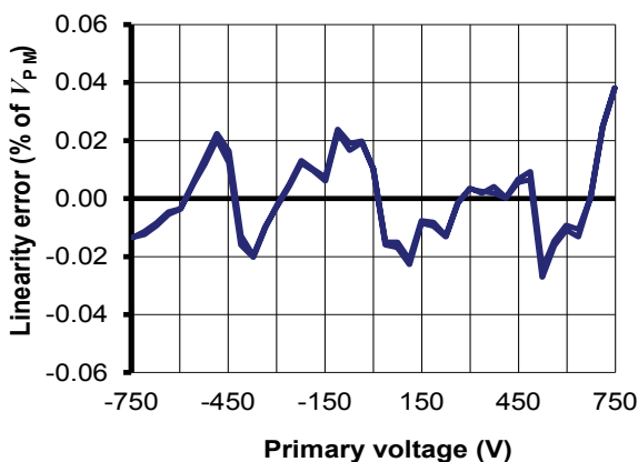
Figure 15: Typical linearity error at 25 °C
