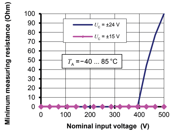
Figure 2: Minimum measuring resistance For T_A under 80 \text{ }^{\circ}\text{C} , the minimum measuring resistance is 0 \text{ } \Omega whatever U_C
