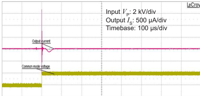
Figure 11: Typical common mode perturbation (2000 V step with 6 kV/μs, R_M = 100 \Omega )
