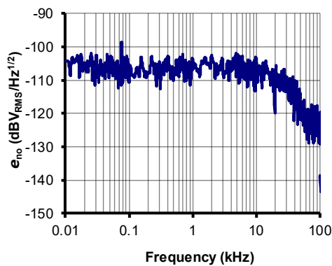
Figure 8: Typical output noise voltage density U_{no} referred to secondary with R_M = 50 \Omega
