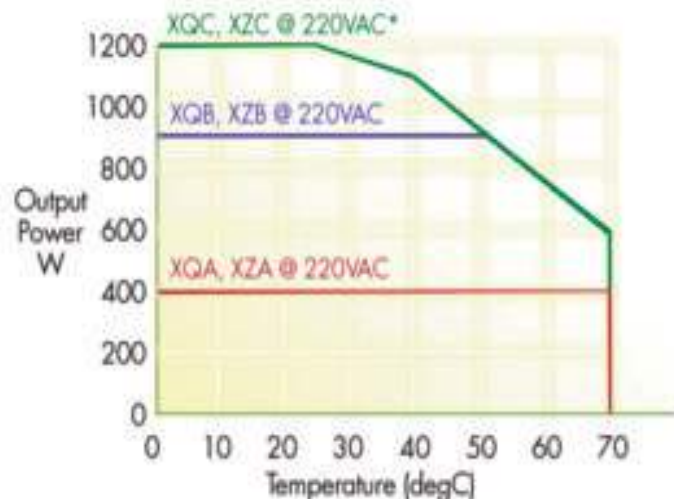
XQA/XQB/XQC and XZA/XZB/XZC @ 220VAC Derating
