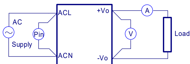
Figure 1. CFM260S Series Test Setup
