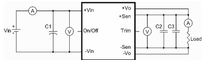
CQB75W8 Series Test Setup
