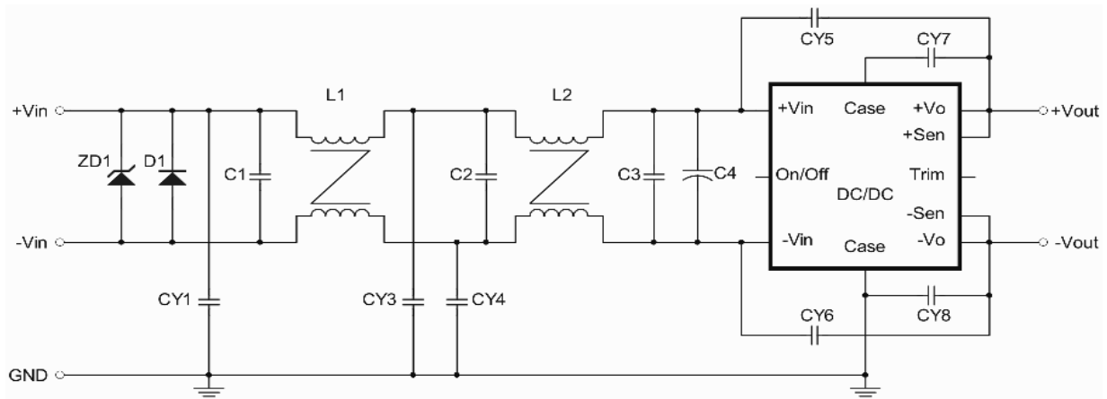
Figure1 Connection circuit
