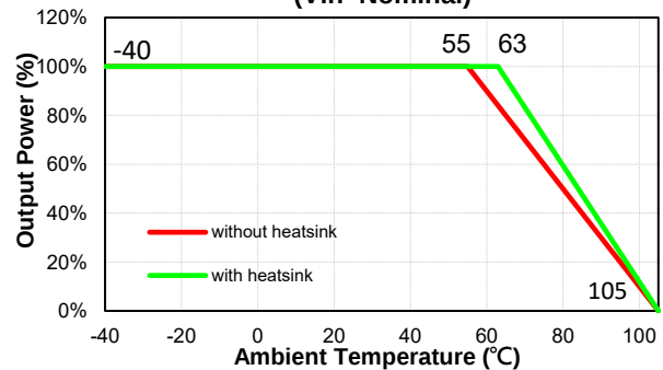
EC5SBW-XXS05 Derating Curve ( V_{in} =Nominal)
