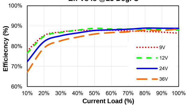
EC5SBW-24S33 Eff Vs Io @25 Deg. C
