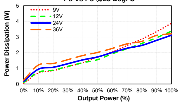
EC5SBW-24S33 Pd Vs Po @25 Deg. C
