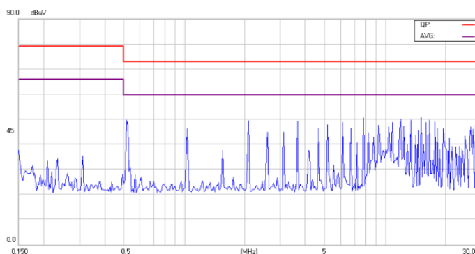
Conducted Class A of EC5SAW-48D15N
