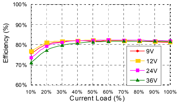
EC5SAW-24S33N (Eff Vs Io)
