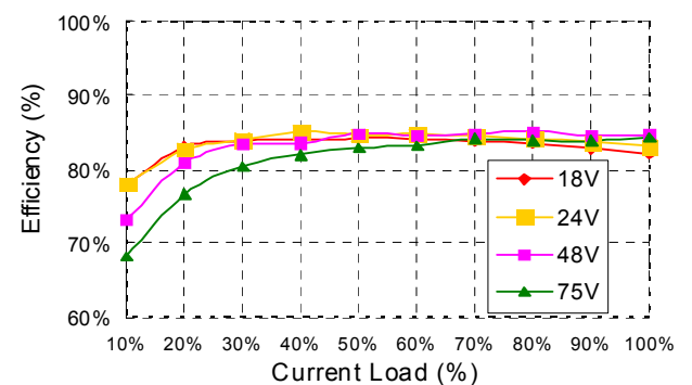
EC5SAW-48D05N (Eff Vs Io)
