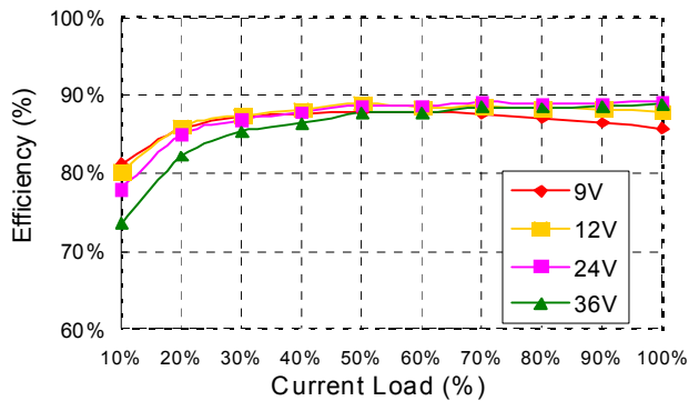
EC5SAW-24D15N (Eff Vs Io)
