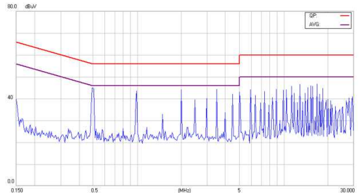
Conducted Class B of EC5SAW -48S15N
