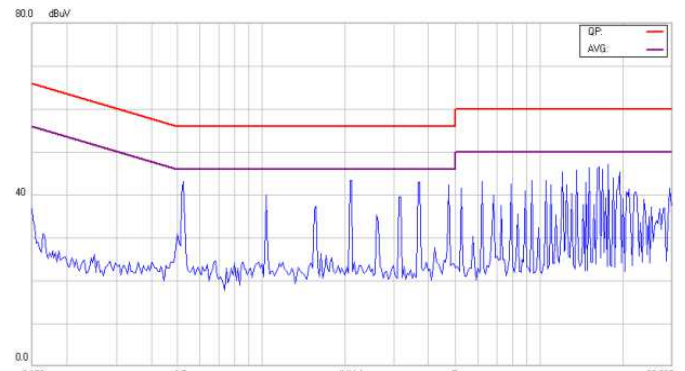
Conducted Class B of EC5SAW-48D12N
