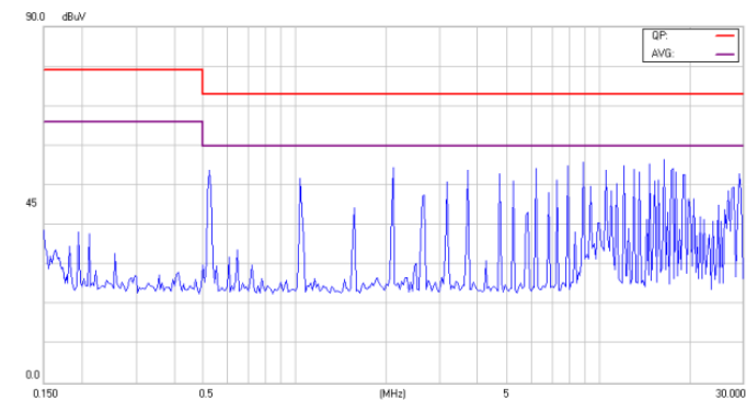
Conducted Class A of EC5SAW-48D12N
