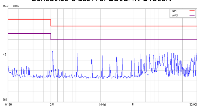
Conducted Class A of EC5SAW -24S05N
