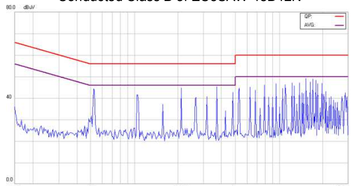
Conducted Class B of of EC5SAW-48D15N
