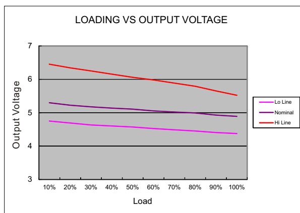
5 Models
