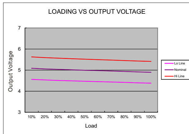
48 Models
