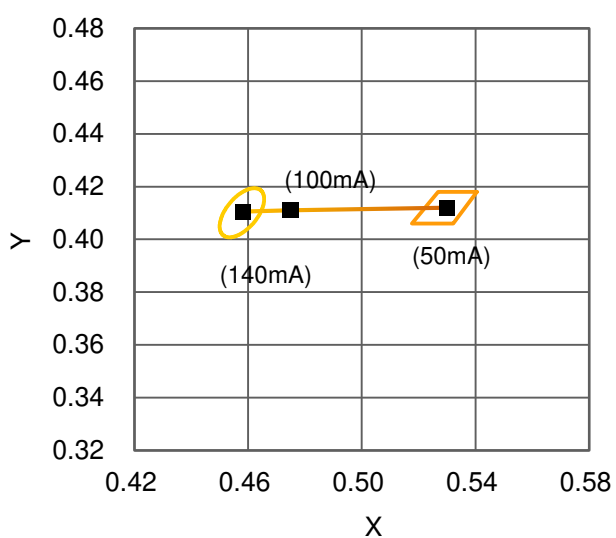
Fig 8. Chromaticity Coordinate Profile at T_C=25^\circ\text{C} .
