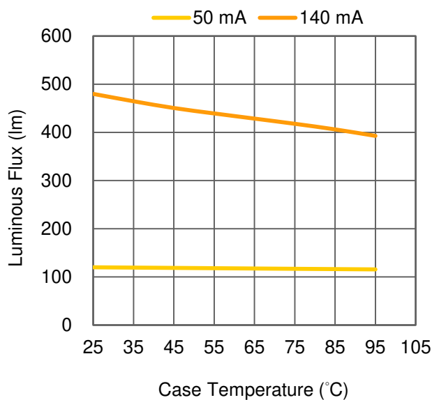
Fig 1. Case Temperature vs. Luminous Flux at 50 mA & 140 mA.
