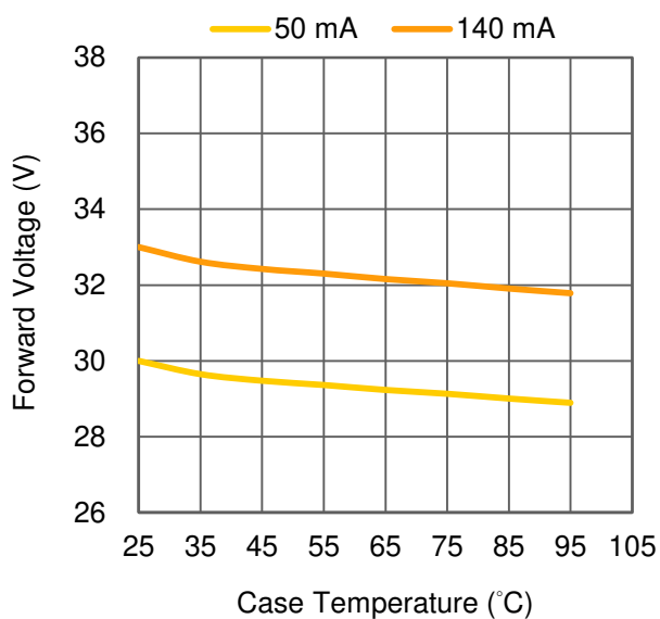
Fig 2. Case Temperature vs. Forward Voltage at 50 mA & 140 mA.
