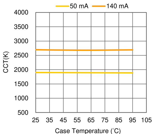
Fig 3. Case Temperature vs. Chromaticity Coordinate \Delta x at 50 mA & 140mA.
