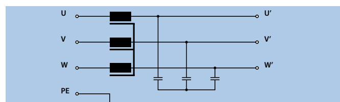
Schematic of a typical sinusoidal filter for solar applications
