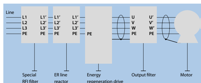
Installation of additional measures for ER drives
