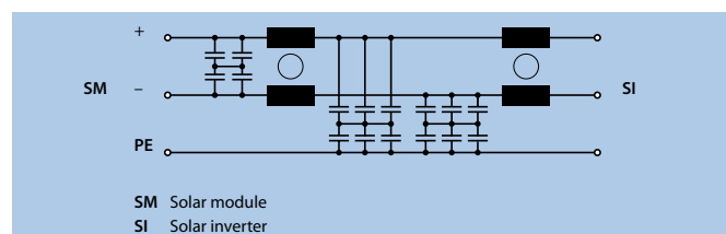
Schematic of a typical DC EMC filter for solar applications
