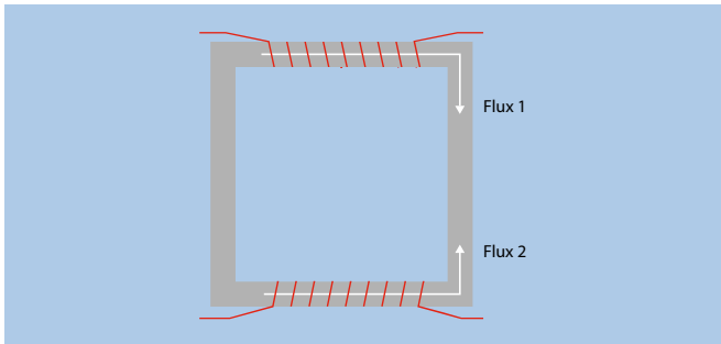
Principle of current compensation
