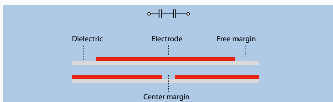
Series construction of capacitors
