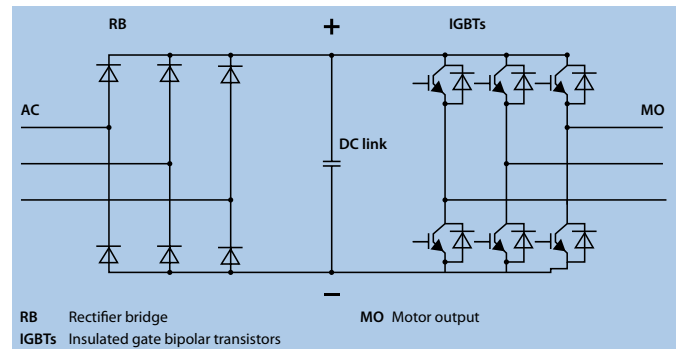
Rectifier bridge in a frequency converter
