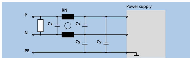
Basic power line filter to remove common and differential-mode noise, based on a current-compensated choke
