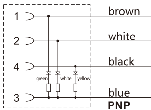
Circuit diagram/电路图
