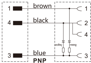
Circuit diagram/电路图
