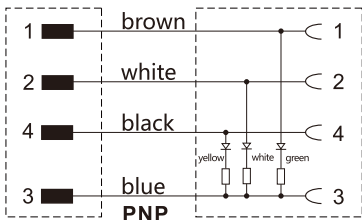
Circuit diagram/电路图
