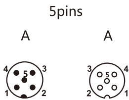
Contact layout/针孔排布 (Front view/前视图)
