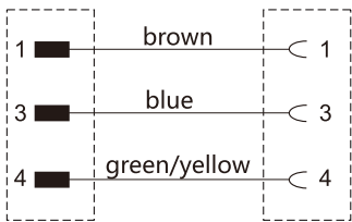
Circuit diagram/电路图
