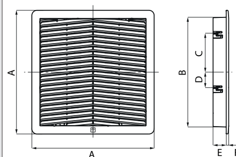
Technical drawing
