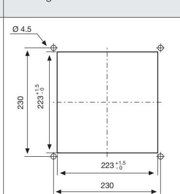
Mounting cut-out
