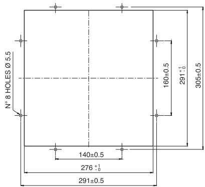
Mounting cut-out
