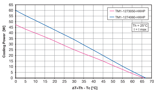
Cooling power vs temperature difference
