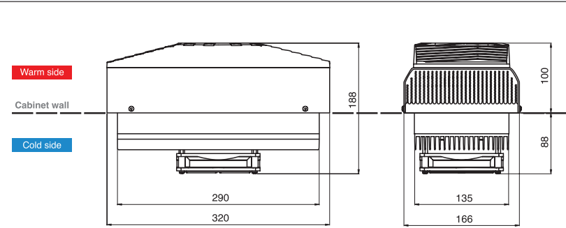
Technical drawing
