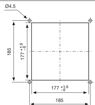
Mounting cut-out
