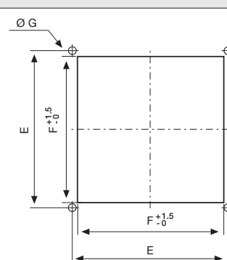
Mounting cut-out
