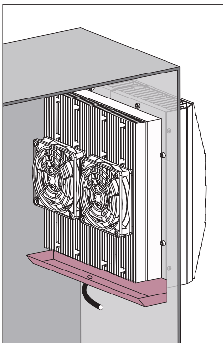
TCU200 / TCU200AC - max. height with drip tray
