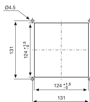
Mounting cut-out
