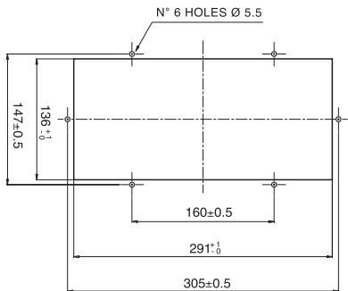
Mounting cut-out
