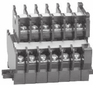
面板組裝 Assembly of Panel Mounting
