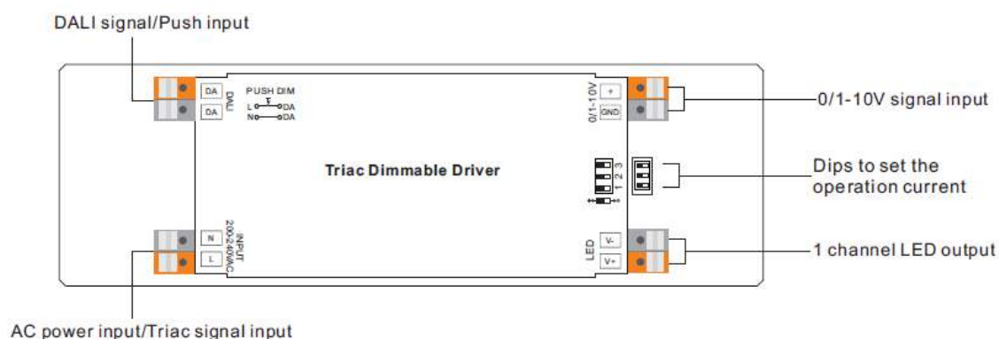
Dips to set the operation current
