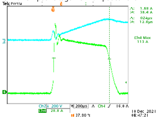
INPUT=230VAC/50HZ @ FULL LOAD CH2: AC Input Voltage CH4: Input current
