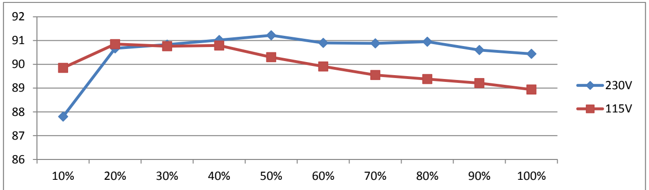
EFFICIENCY vs LOAD
