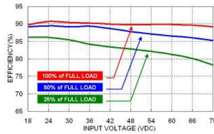
RCD20-48S05W Efficiency vs. Input Voltage
