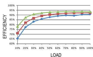
RSD-150D-12
