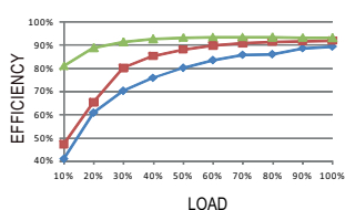
RSD-150C-12
