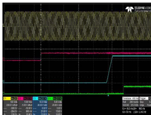
Figure 14: CNS655-MU Turn-on delay by Inhibit – V_{IN} = 90\text{Vac} Load: I_O = 16.7\text{A} , I_{SB} = 1\text{A} Ch 1: V_{IN} Ch 2: Inhibit Ch 3: V_O Ch 4: PWOK
