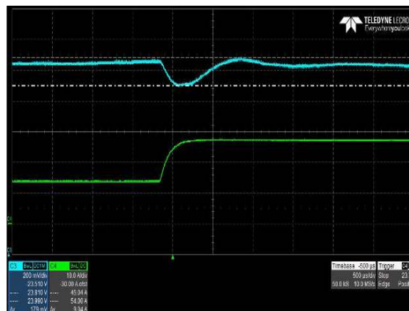
Figure 20: CNS655-MU Transient Response – V_o Deviation (Low to High) V_{IN} = 90V_{ac} , I_o = 50\% to 100% load, Output Cap = 330 \mu F/A Ch 3: V_o Ch 4: I_o
