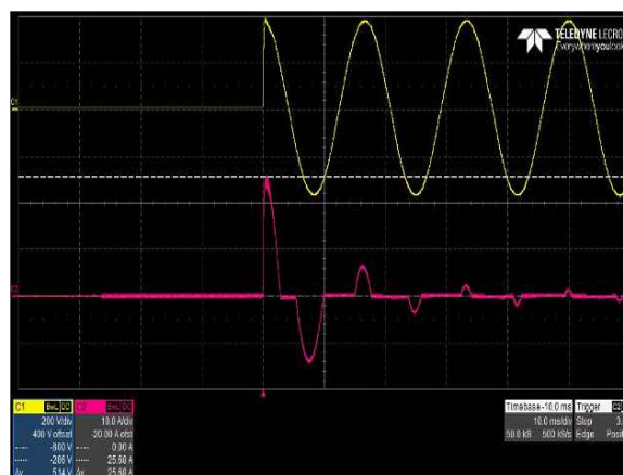
Figure 18: CNS655-MU Inrush Current – V_{in} = 264\text{Vac} Load: I_O = 0\text{A} , Turn on Angle = 90^\circ Ch 1: V_{IN} Ch 2: I_{IN}
