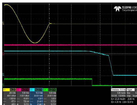
Figure 16: CNS655-MU Hold-up Time – V_{in} = 264\text{Vac} / 47\text{Hz} / 0^\circ Load: I_O = 16.7\text{A} , I_{SB} = 1\text{A} Ch 1: V_{IN} Ch 2: V_{SB} Ch 3: V_O Ch 4: PWOK
