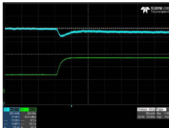
Figure 8: CNS653-ME Transient Response – V_o Deviation (Low to High) V_{IN} = 90\text{Vac} , I_o = 50\% to 100% load, Output Cap = 330 \mu\text{F} /A Ch 3: V_o Ch 4: I_o
