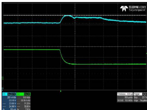
Figure 19: CNS655-MU Transient Response – V_o Deviation (High to Low) V_{IN} = 90V_{ac} , I_o = 100\% to 50% load, Output Cap = 330 \mu F/A Ch 3: V_o Ch 4: I_o
