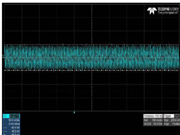
Figure 21: CNS655-MU Ripple and Noise Measurement – V_{IN} = 115V_{ac} Load: I_o = 16.7A Ch 3: V_o
