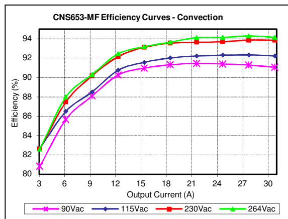
Figure 12: CNS653-MF Efficiency Curves @ 25°C, Convection Cool V_{IN} = 90 to 264Vac, Load: I_o = 0 to 30.8A
