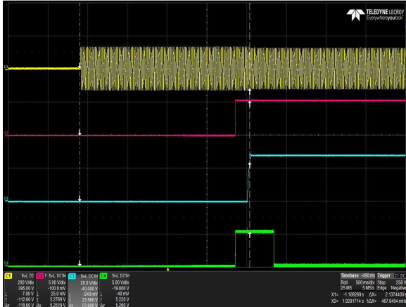
Figure 34: LCM1500R-T-4 Turn-on delay via AC mains Vin = 90Vac Load: Io = 53.6A (28V), Isb = 2A (5V) Ch 1: Vin Ch 2: Vsb Ch 3: Vo Ch 4: G_DCOK_C
