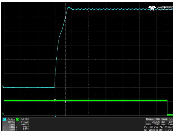
Figure 38: LCM1500R-T-4 Output Voltage Startup Vin = 90Vac Load: Io = 53.6A (28V), Isb = 2A (5V) Ch 3: Vo Ch 4: G_DCOK_C
