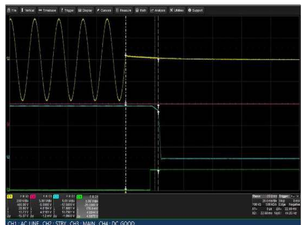
Figure 6: LCM3000L-T Hold-up Time
