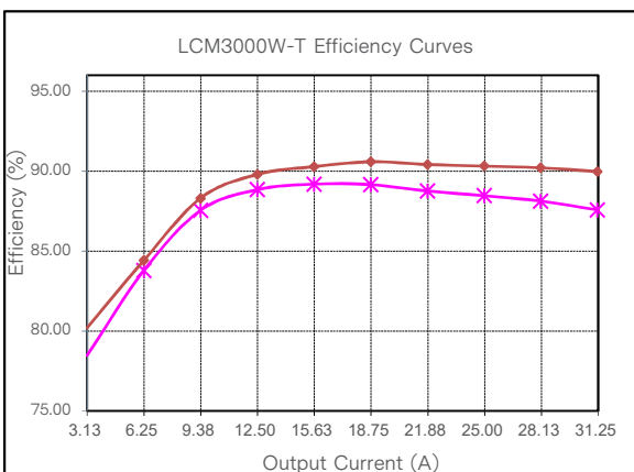
Figure 53: LCM3000W-T Efficiency Curve @ 25°C Loading: I_{o\_min} = 10\%I_{o\_max} increment to 31.25A, I_{sb} = 0A
