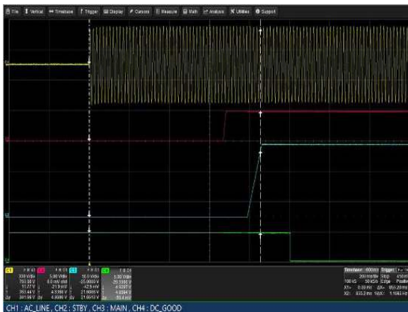
Figure 17: LCM3000Q-T Turn-on delay via AC mains
