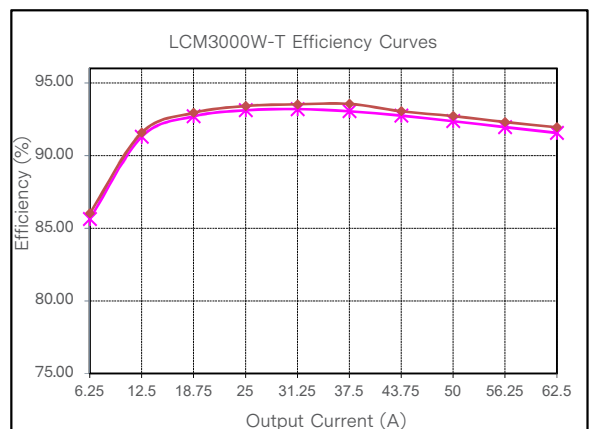
Figure 54: LCM3000W-T Efficiency Curve @ 25°C Loading: I_{o\_min} = 10\%I_{o\_max} increment to 62.5A, I_{sb} = 0A
