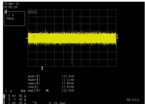
Figure 10: LCM600L Ripple and Noise Measurement V_{in} = 90V_{ac} Load: I_o = 50A (12V), I_{SB} = 2A (5V) Ch 1: V_o
