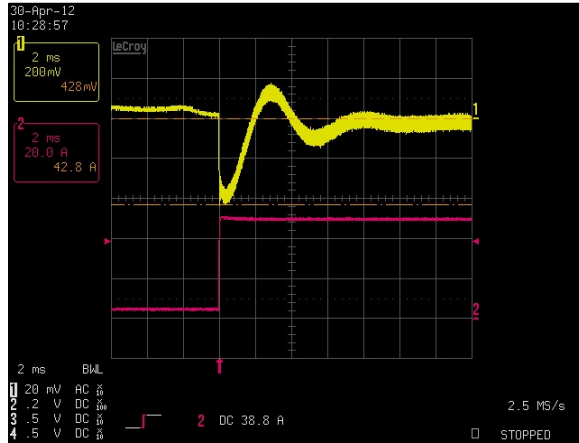
Figure 7: LCM600L Transient Response - V_o Deviation 10% to 100% load change 1A/uS slew rate V_{in} = 230V_{ac} Ch 1: V_o Ch 2: I_o
