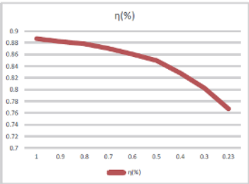
Eff. Vs load
