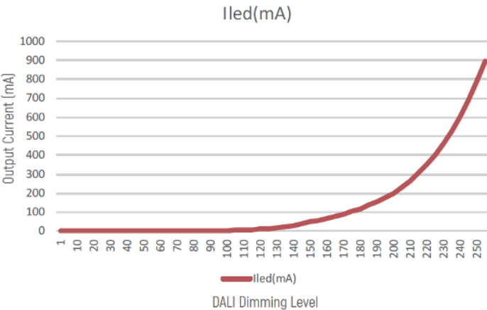
Dimming curve
