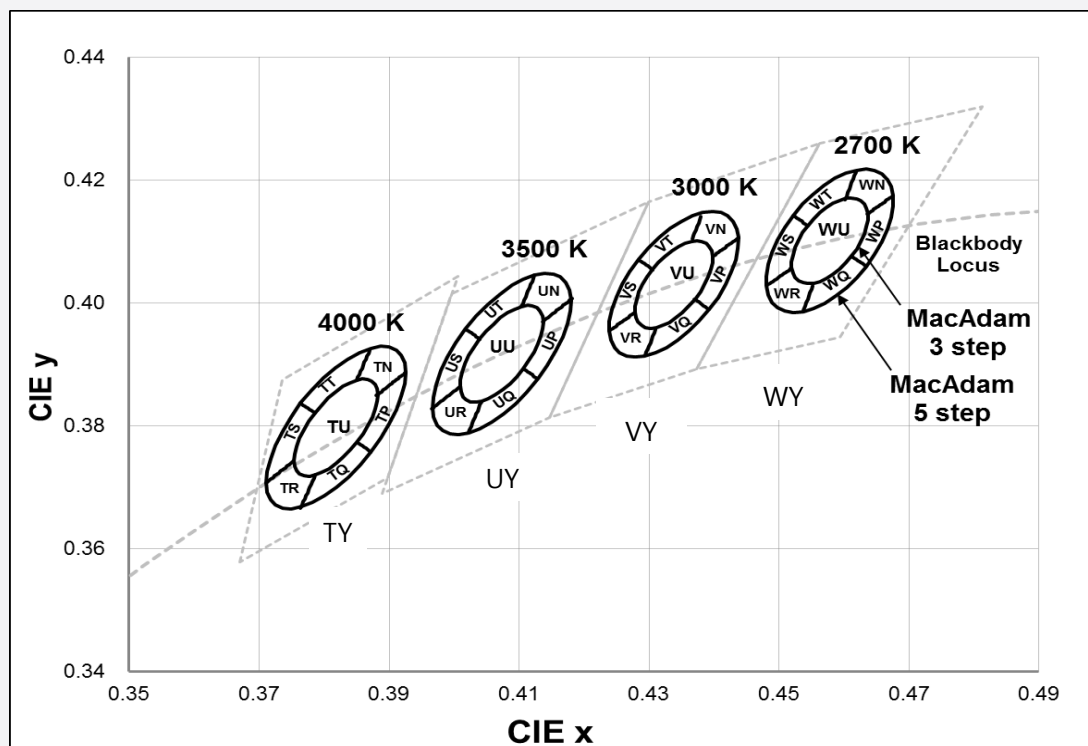
f) Chromaticity Region & Coordinates for Y kitting bin or mac3 only bin ( I_F = 65 mA, T_a = 25 °C)
