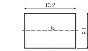
Dimension Drawing “/THT” version (mm)
