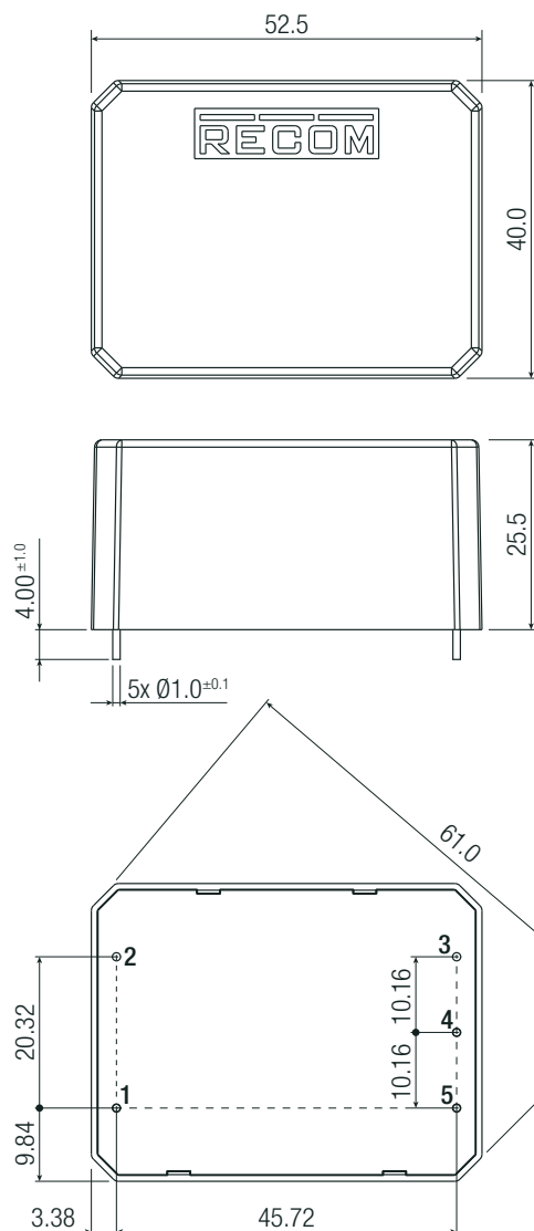
Dimension Drawing “/277” version SINGLE and DUAL Output (mm)
