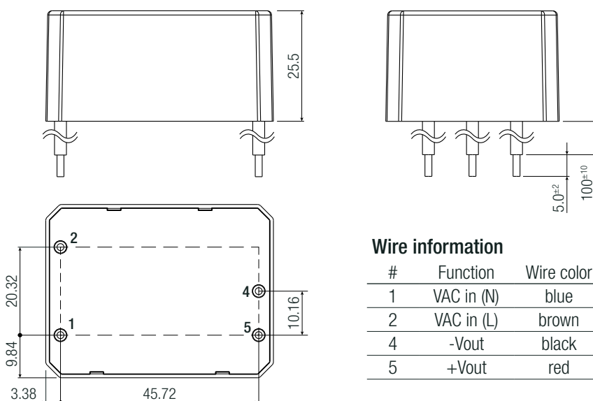
Dimension Drawing Wired version “/W” SINGLE Output (mm)
