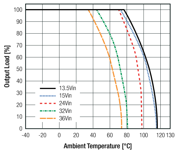
Thermal Derating
