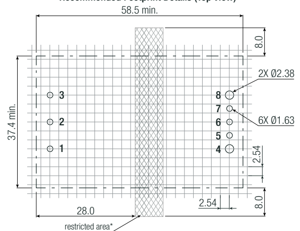
Recommended Footprint Details (Top View)
