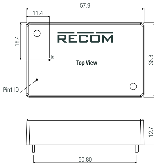
Dimension Drawing (mm)
