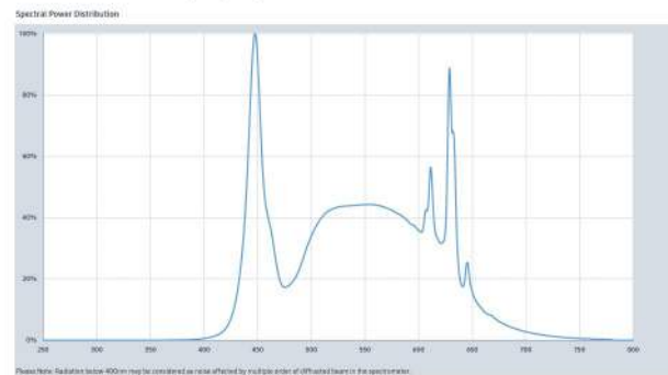
Samsung MPL 2835 LM281B+ PRO S90 VK, VL, S90, 5700K
