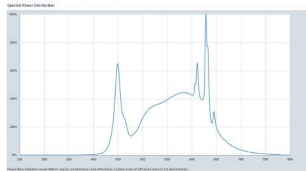
Samsung MPL 2835 LM281B+ PRO S90 VK, VL, S90, 4000K
