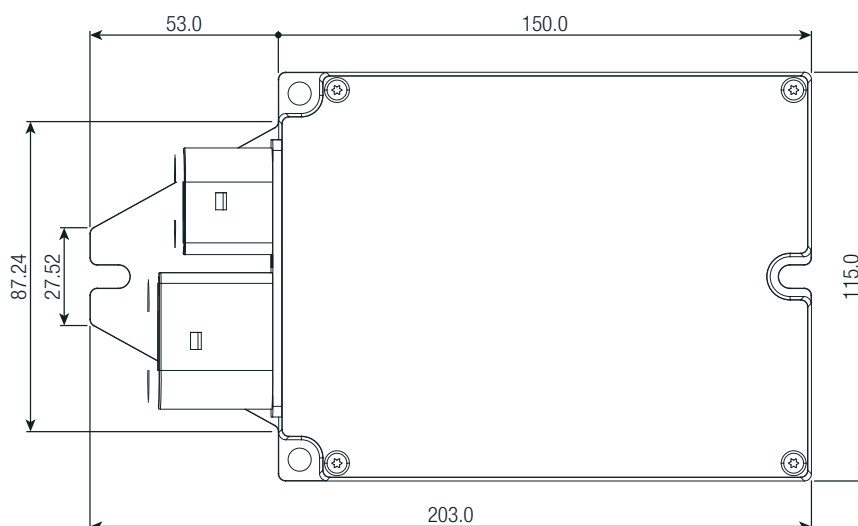
Dimension Drawing RMOD400-28-13SW (mm)
