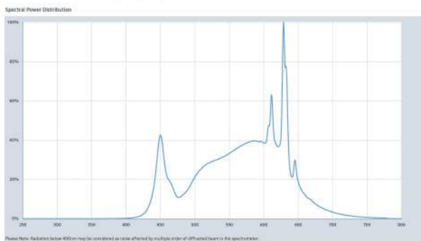
Samsung MPL 2835 LM281B+ PRO S90 VK, VL, S90, 3500K
