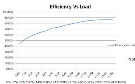
Driver Performance
