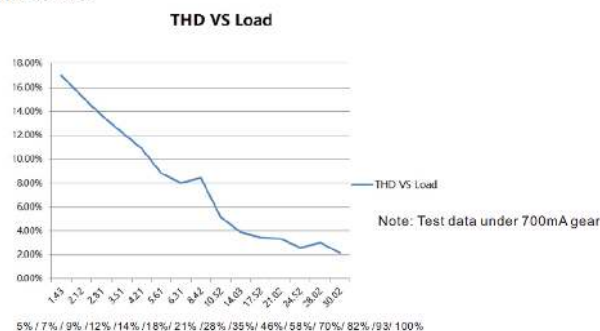
Driver Performance
