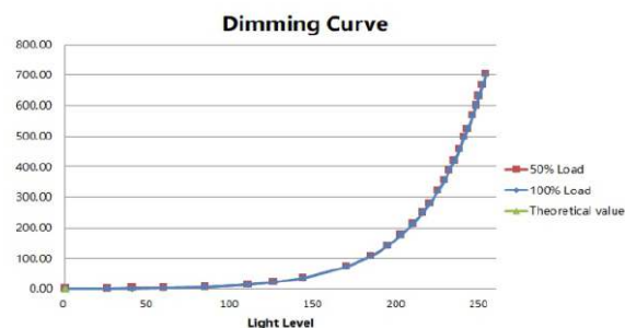
Dimming Curve
