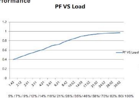
Driver Performance
