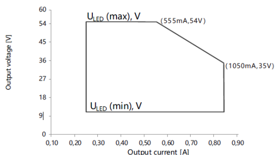
Driver Performance
