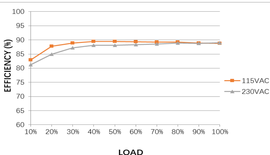
EFFICIENCY vs LOAD
