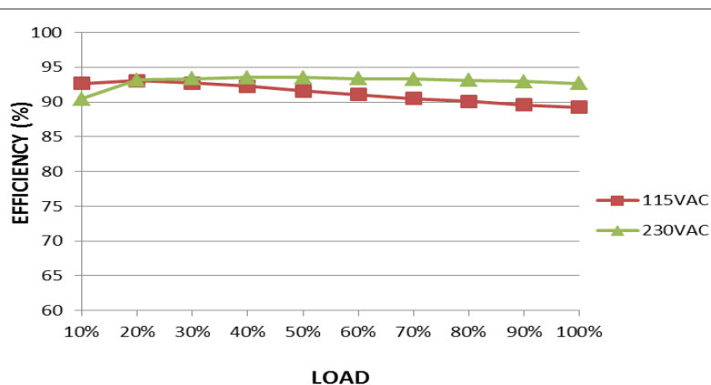
EFFICIENCY vs LOAD
