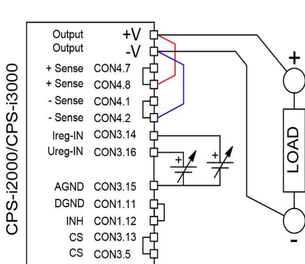
Standard Configuration
